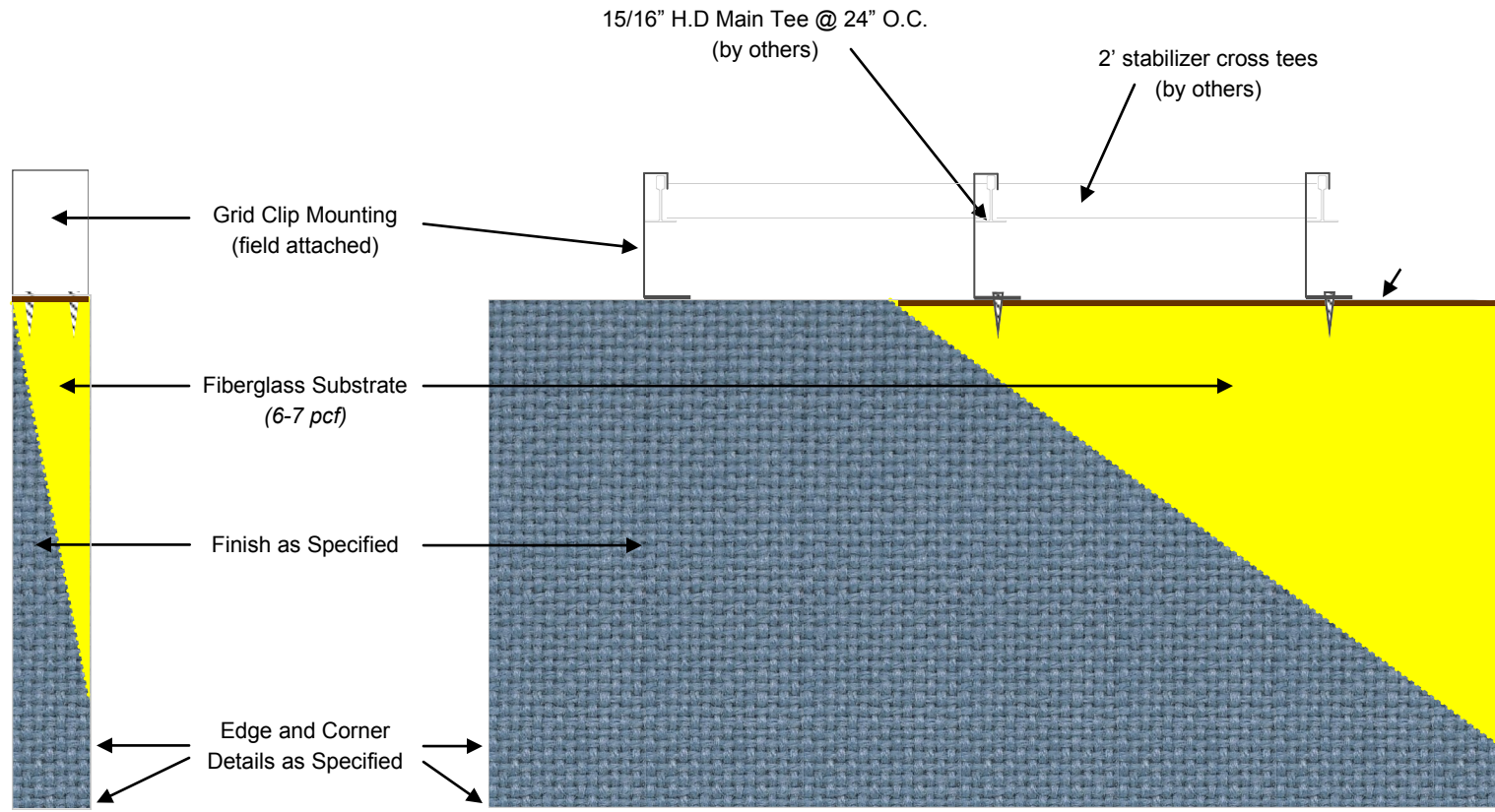
PANEL SECTION
